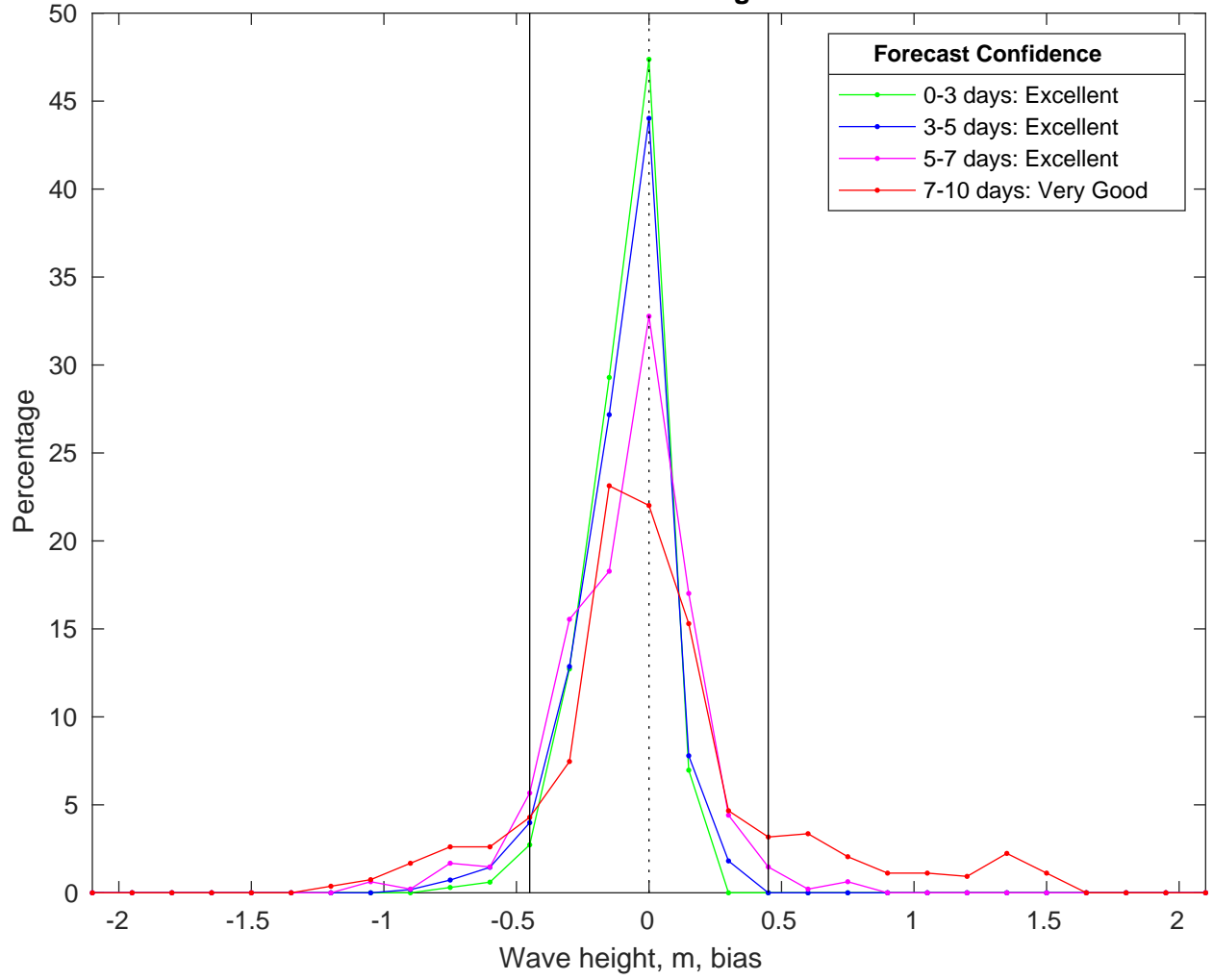
NDBC 42084 vs CMEMS Waves Bias Histogram: 09-Feb-2025
