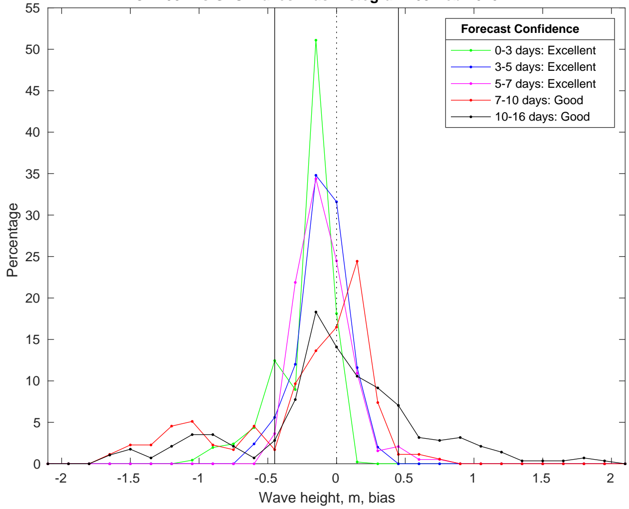
NDBC 42084 vs GFS Waves Bias Histogram: 09-Feb-2025
