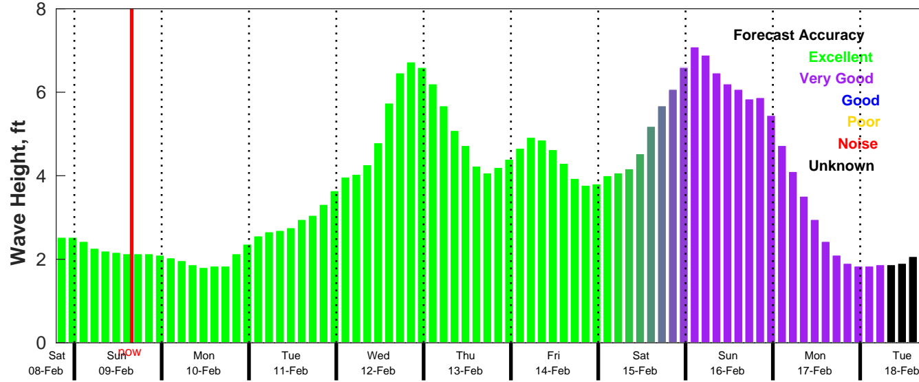
CMEMS Wave Forecast for NDBC 42084 from 08-Feb-2025 19:00:00 to 18-Feb-2025 19:00:00
