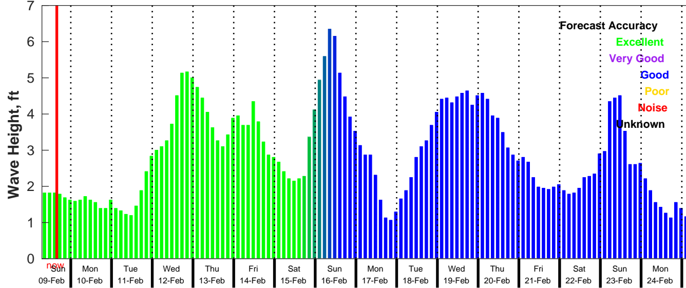
GFS Wave Forecast for NDBC 42084 from 09-Feb-2025 07:00:00 to 25-Feb-2025 07:00:00
