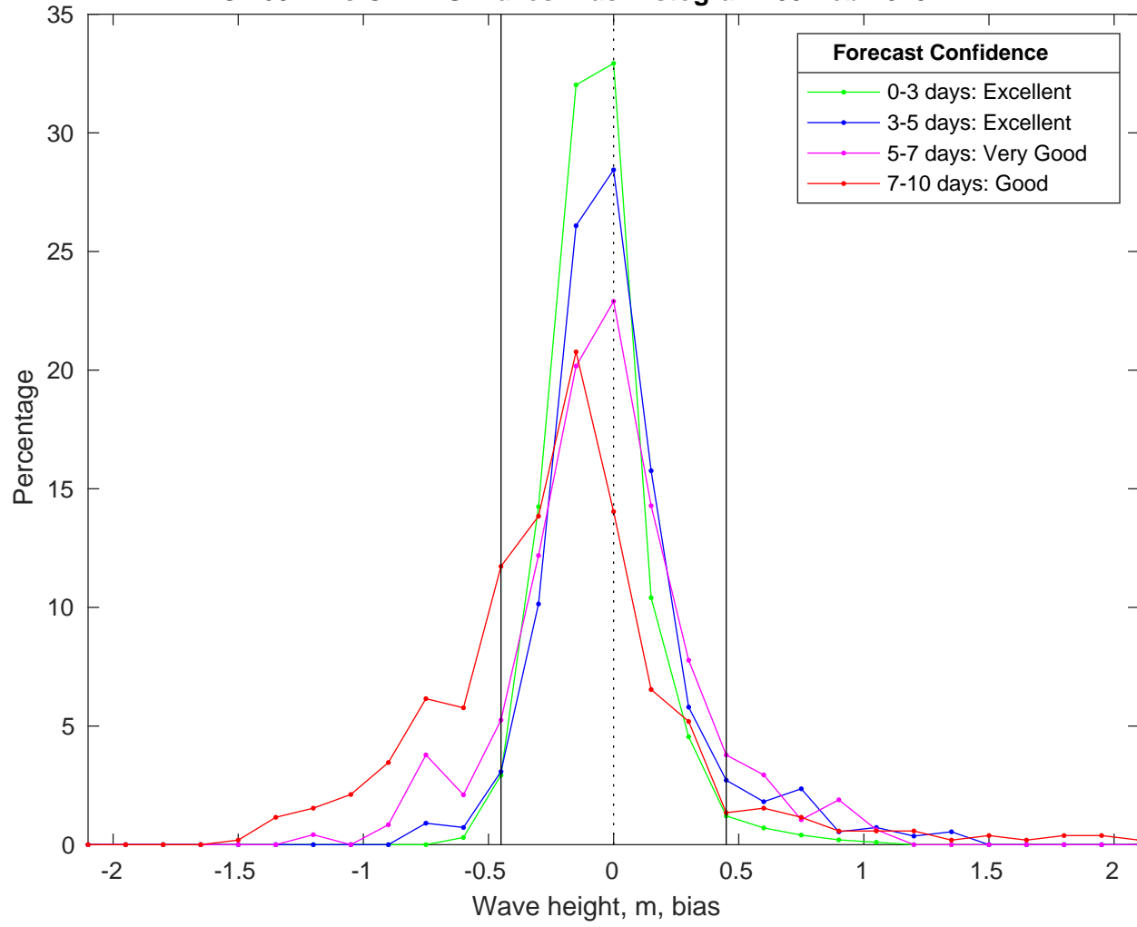
NDBC 46011 vs CMEMS Waves Bias Histogram: 09-Feb-2025
