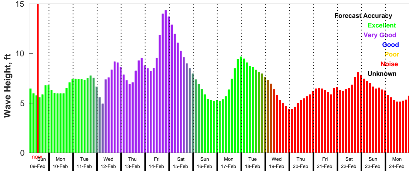
GFS Wave Forecast for NDBC 46011 from 09-Feb-2025 04:00:00 to 25-Feb-2025 04:00:00
