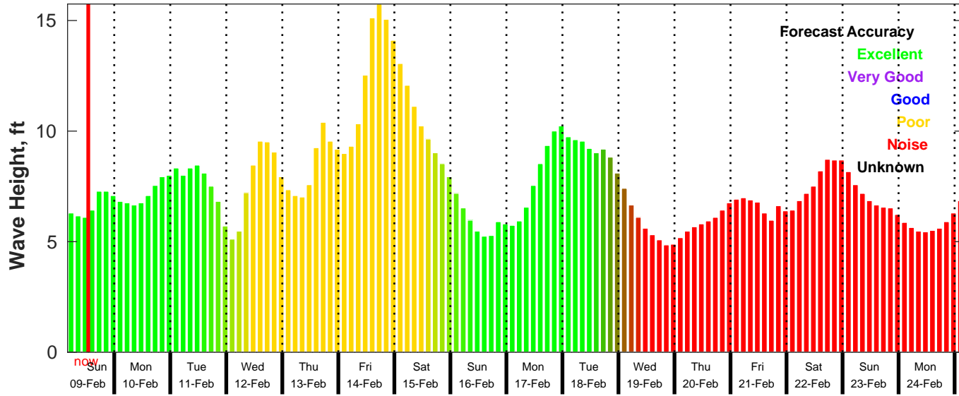
GFS Wave Forecast for NDBC 46028 from 09-Feb-2025 04:00:00 to 25-Feb-2025 04:00:00
