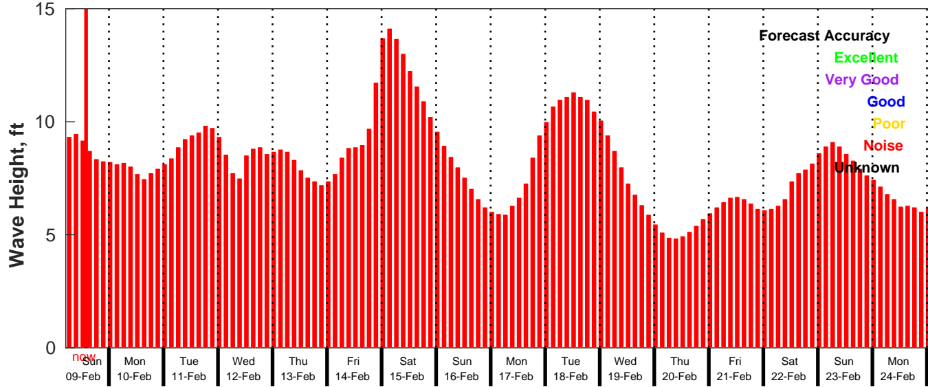
GFS Wave Forecast for NDBC 46053 from 09-Feb-2025 05:00:00 to 25-Feb-2025 05:00:00
