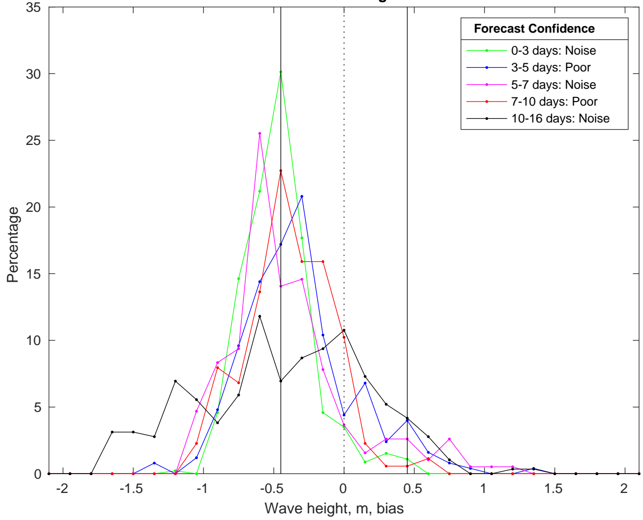
NDBC 46054 vs GFS Waves Bias Histogram: 09-Feb-2025
