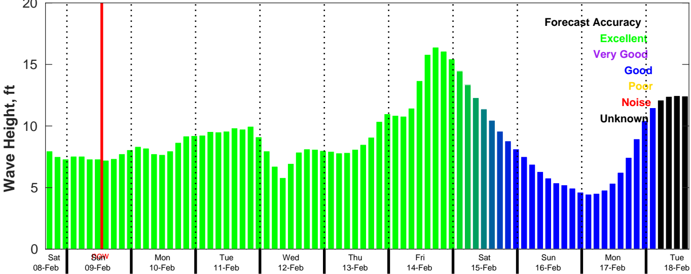
CMEMS Wave Forecast for NDBC 46054 from 08-Feb-2025 16:00:00 to 18-Feb-2025 16:00:00
