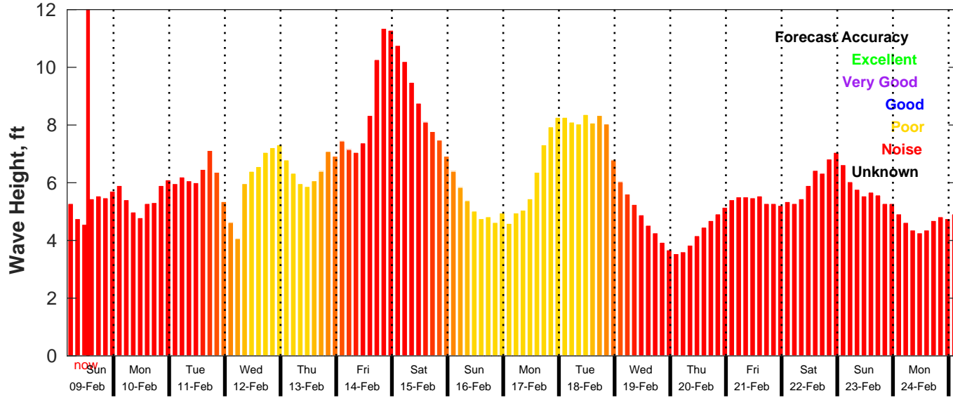
GFS Wave Forecast for NDBC 46054 from 09-Feb-2025 04:00:00 to 25-Feb-2025 04:00:00
