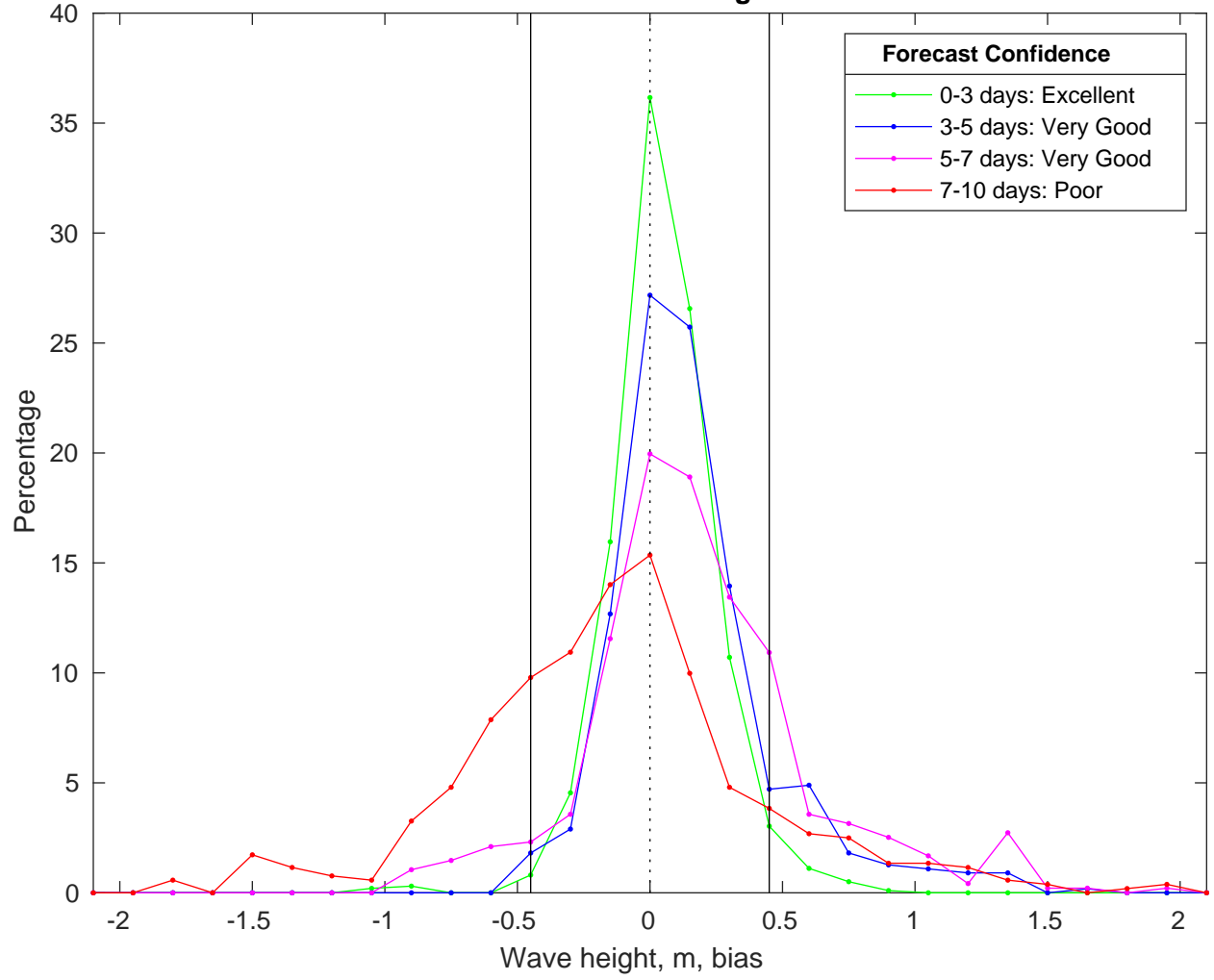
NDBC 46069 vs CMEMS Waves Bias Histogram: 09-Feb-2025
