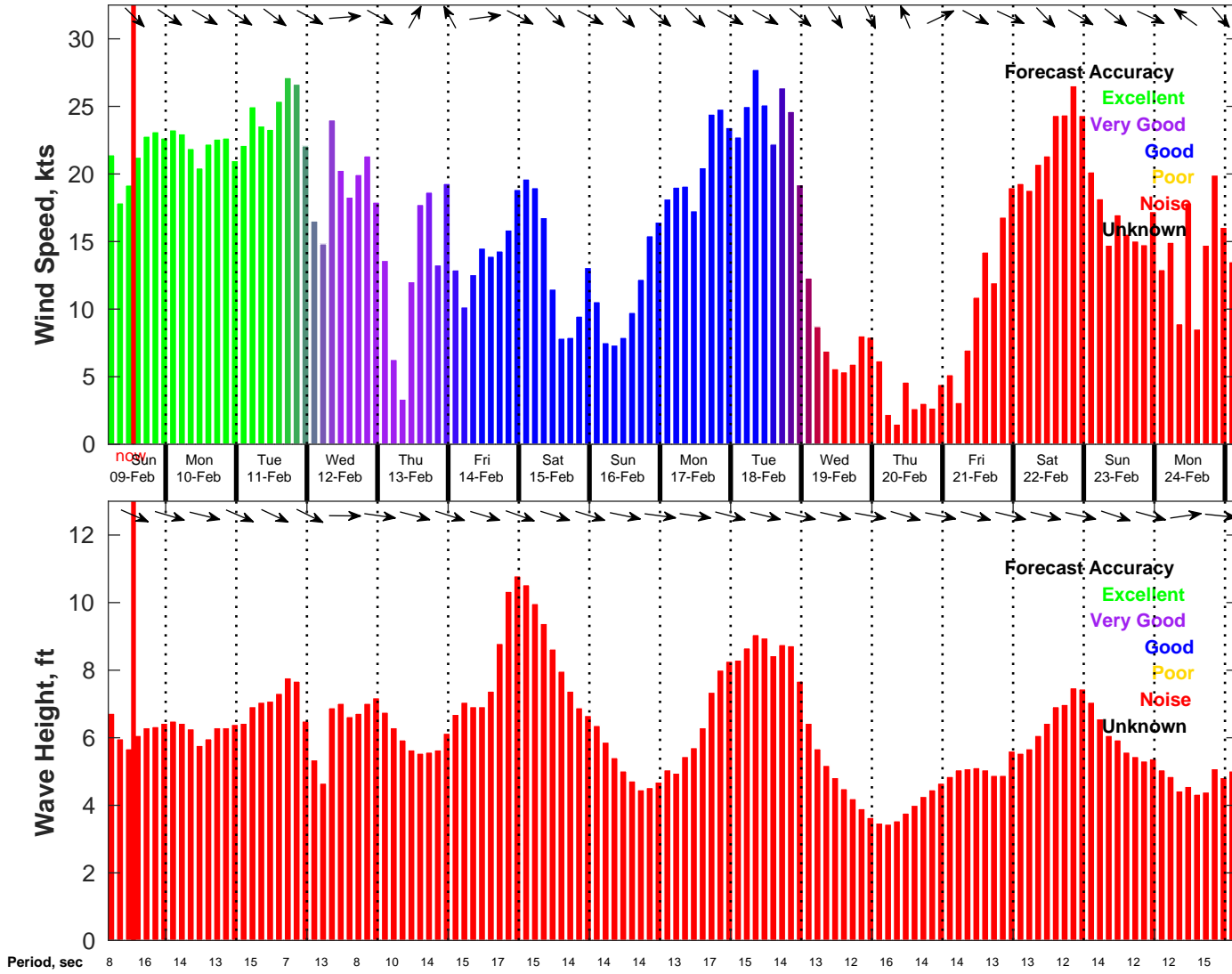
Wind & Wave Forecast for NDBC 46069 from 09-Feb-2025 04:00:00 to 25-Feb-2025 04:00:00
