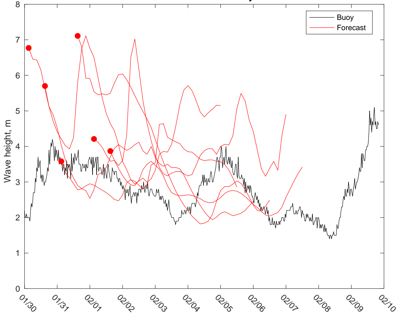
NDBC 46246 vs GFS Waves: 10 to 16 day forecast
