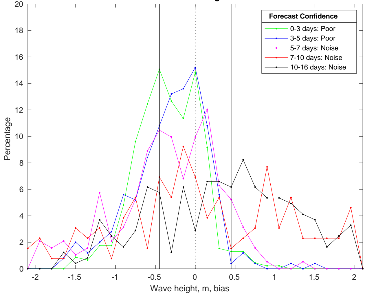
NDBC 46246 vs GFS Waves Bias Histogram: 09-Feb-2025
