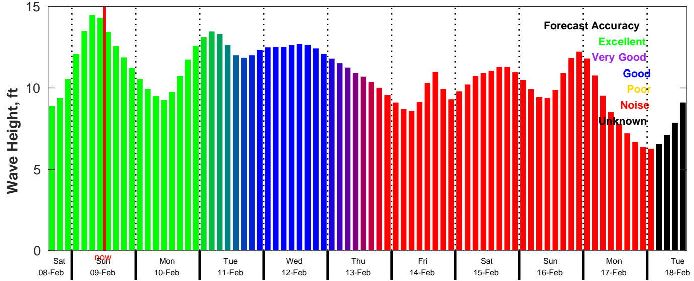
CMEMS Wave Forecast for NDBC 46246 from 08-Feb-2025 15:00:00 to 18-Feb-2025 15:00:00
