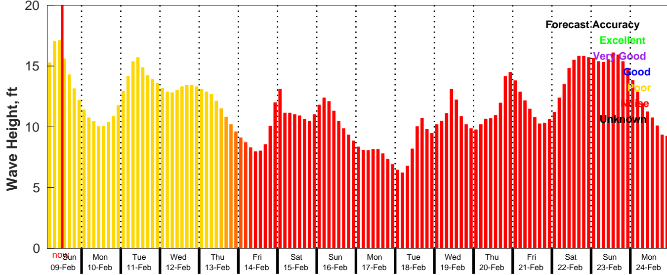
GFS Wave Forecast for NDBC 46246 from 09-Feb-2025 03:00:00 to 25-Feb-2025 03:00:00
