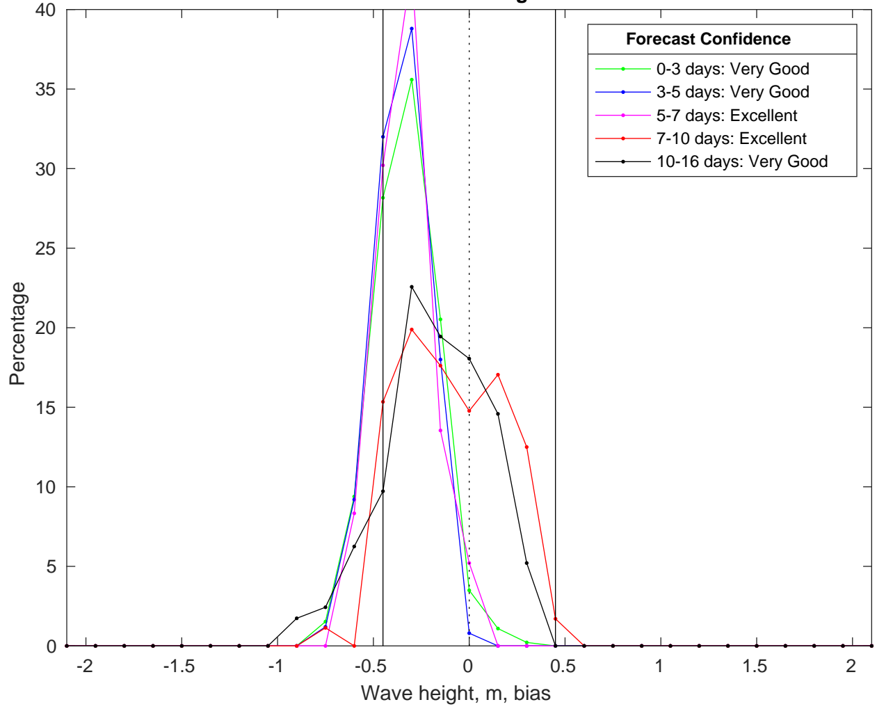
NDBC 51209 vs GFS Waves Bias Histogram: 09-Feb-2025
