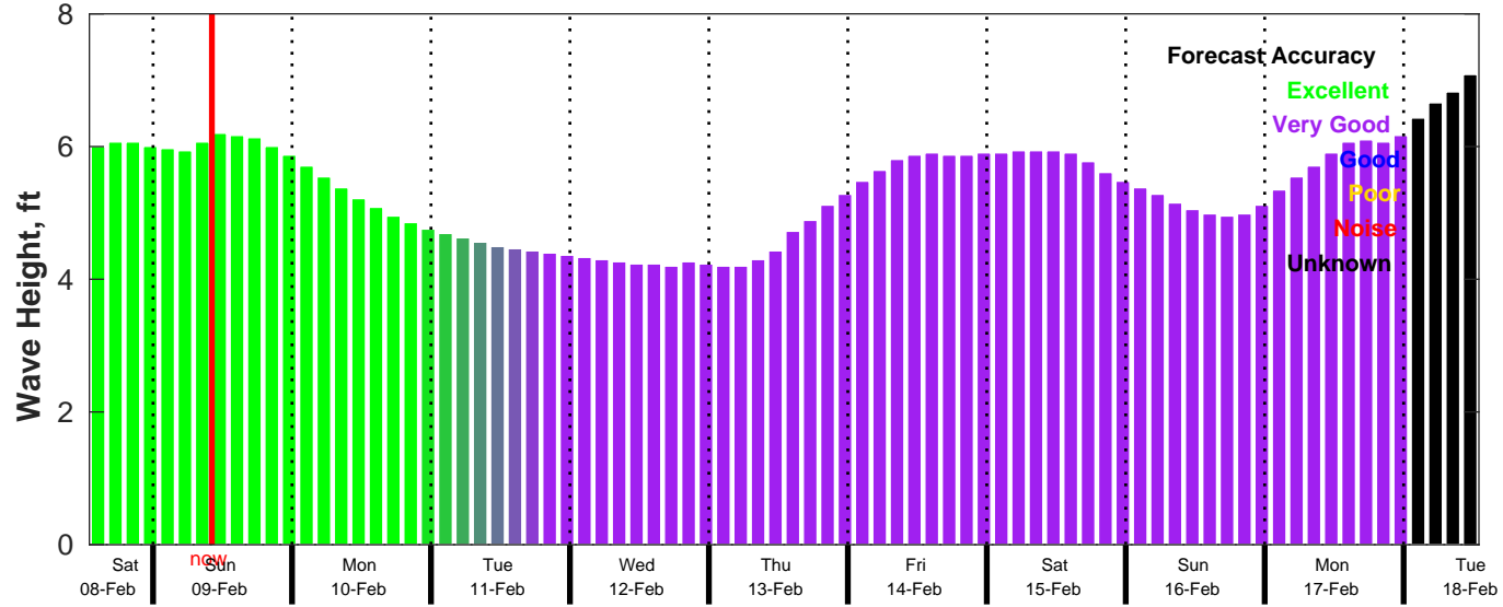
CMEMS Wave Forecast for NDBC 51209 from 08-Feb-2025 13:00:00 to 18-Feb-2025 13:00:00
