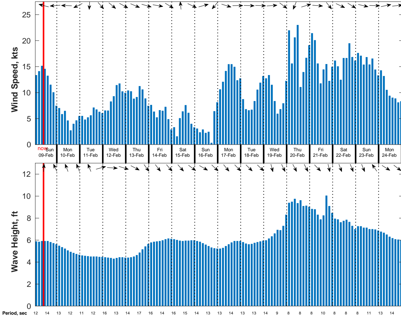
Wind & Wave Forecast for NDBC 51209 from 09-Feb-2025 01:00:00 to 25-Feb-2025 01:00:00
