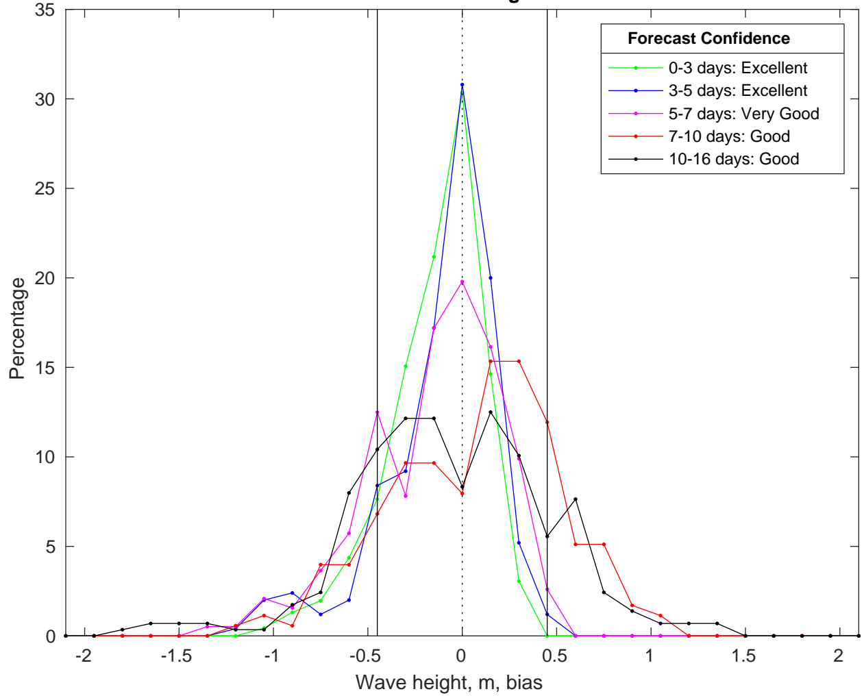
NDBC 52211 vs GFS Waves Bias Histogram: 09-Feb-2025
