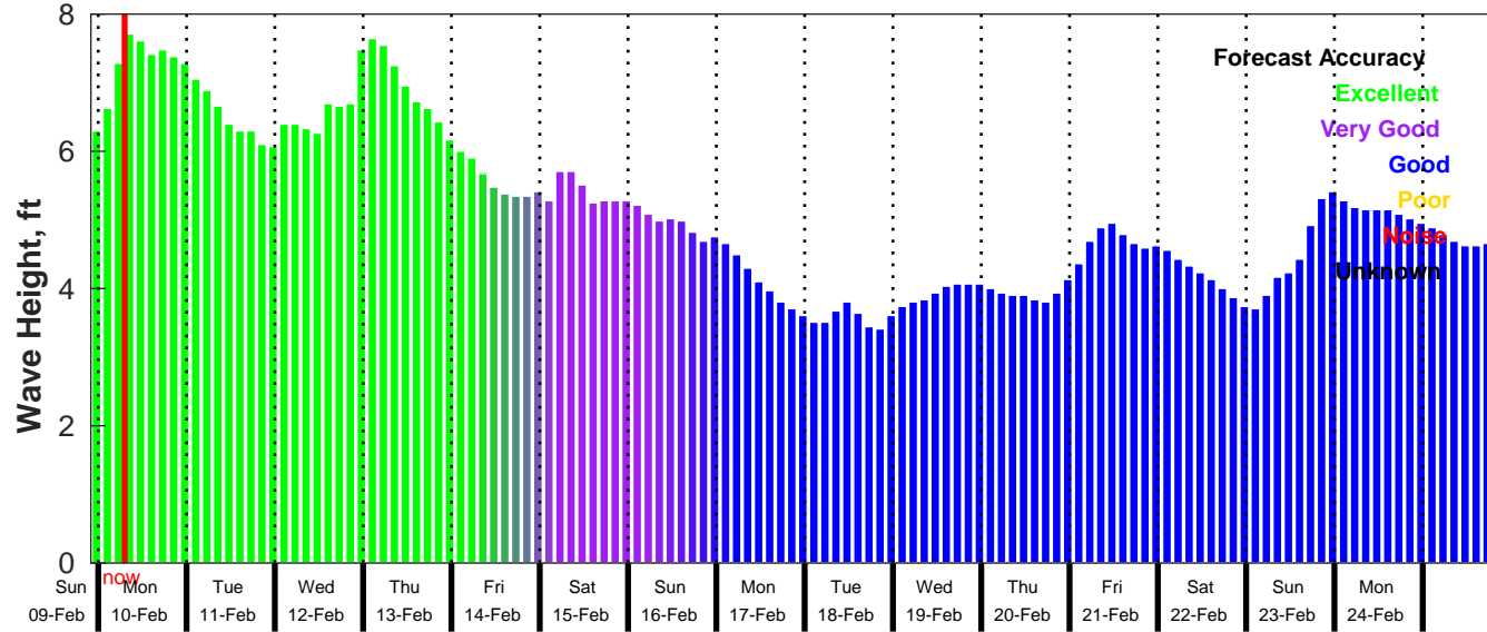
GFS Wave Forecast for NDBC 52211 from 09-Feb-2025 22:00:00 to 25-Feb-2025 22:00:00
