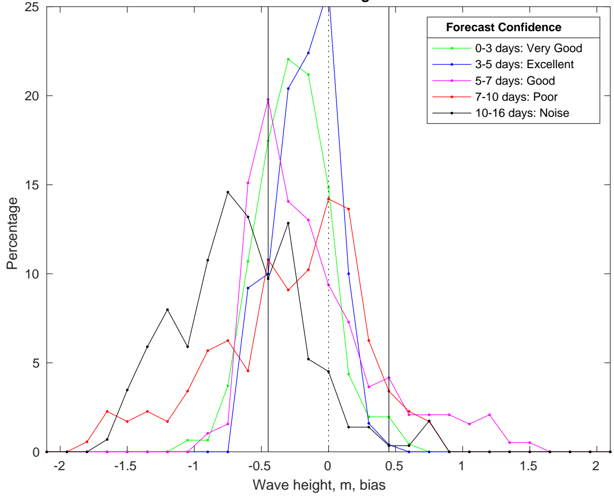
NDBC 52212 vs GFS Waves Bias Histogram: 09-Feb-2025
