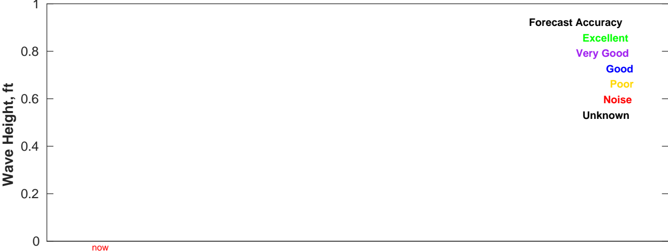
CMEMS Wave Forecast for NDBC 52212 from 09-Feb-2025 09:00:00 to 19-Feb-2025 09:00:00
