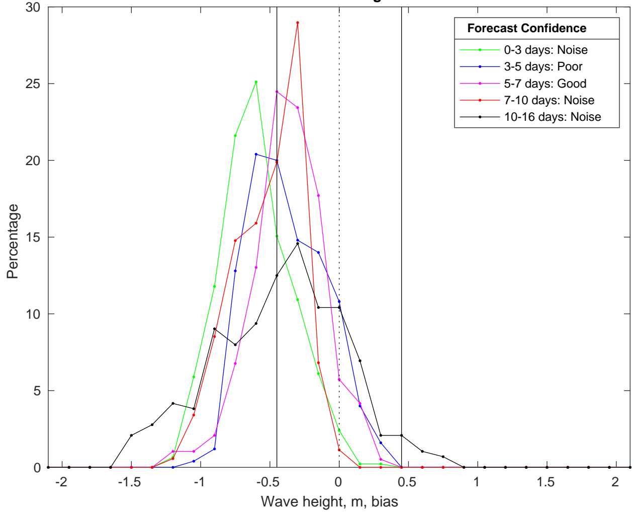
NDBC 52213 vs GFS Waves Bias Histogram: 09-Feb-2025
