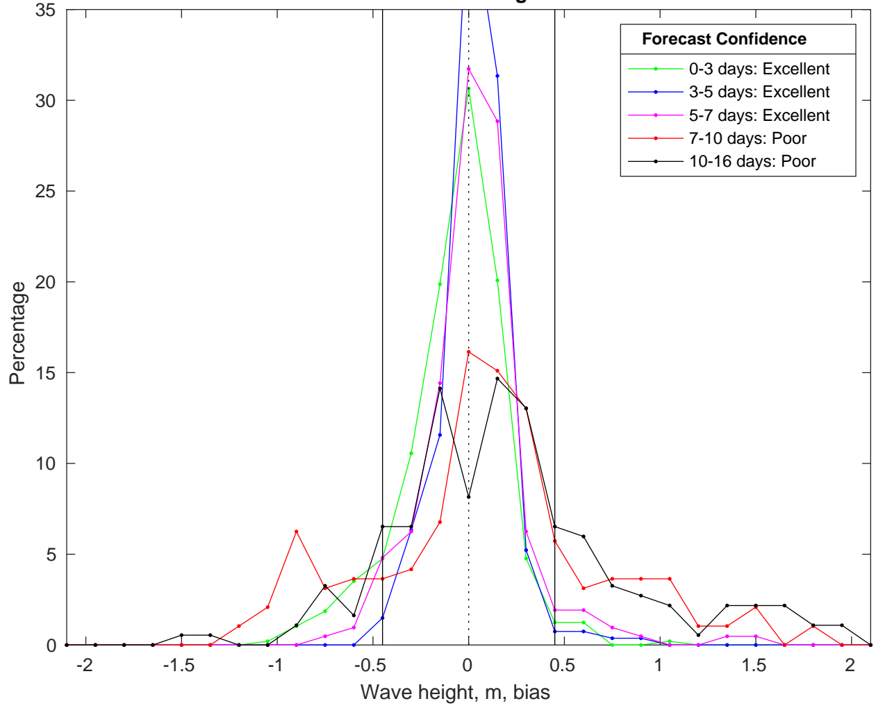
NDBC 41004 vs GFS Waves Bias Histogram: 10-Feb-2025
