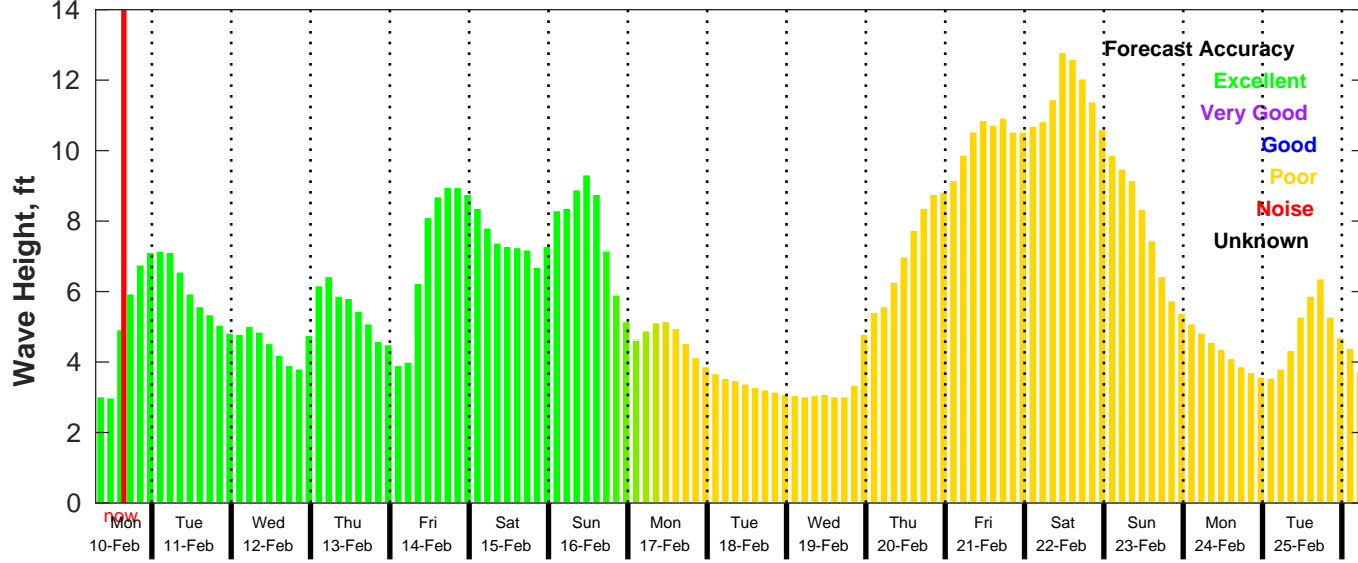
GFS Wave Forecast for NDBC 41004 from 10-Feb-2025 07:00:00 to 26-Feb-2025 07:00:00
