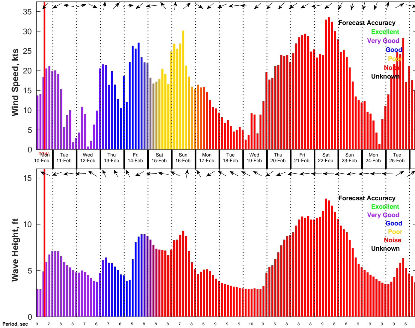
Wind & Wave Forecast for NDBC 41004 from 10-Feb-2025 07:00:00 to 26-Feb-2025 07:00:00
