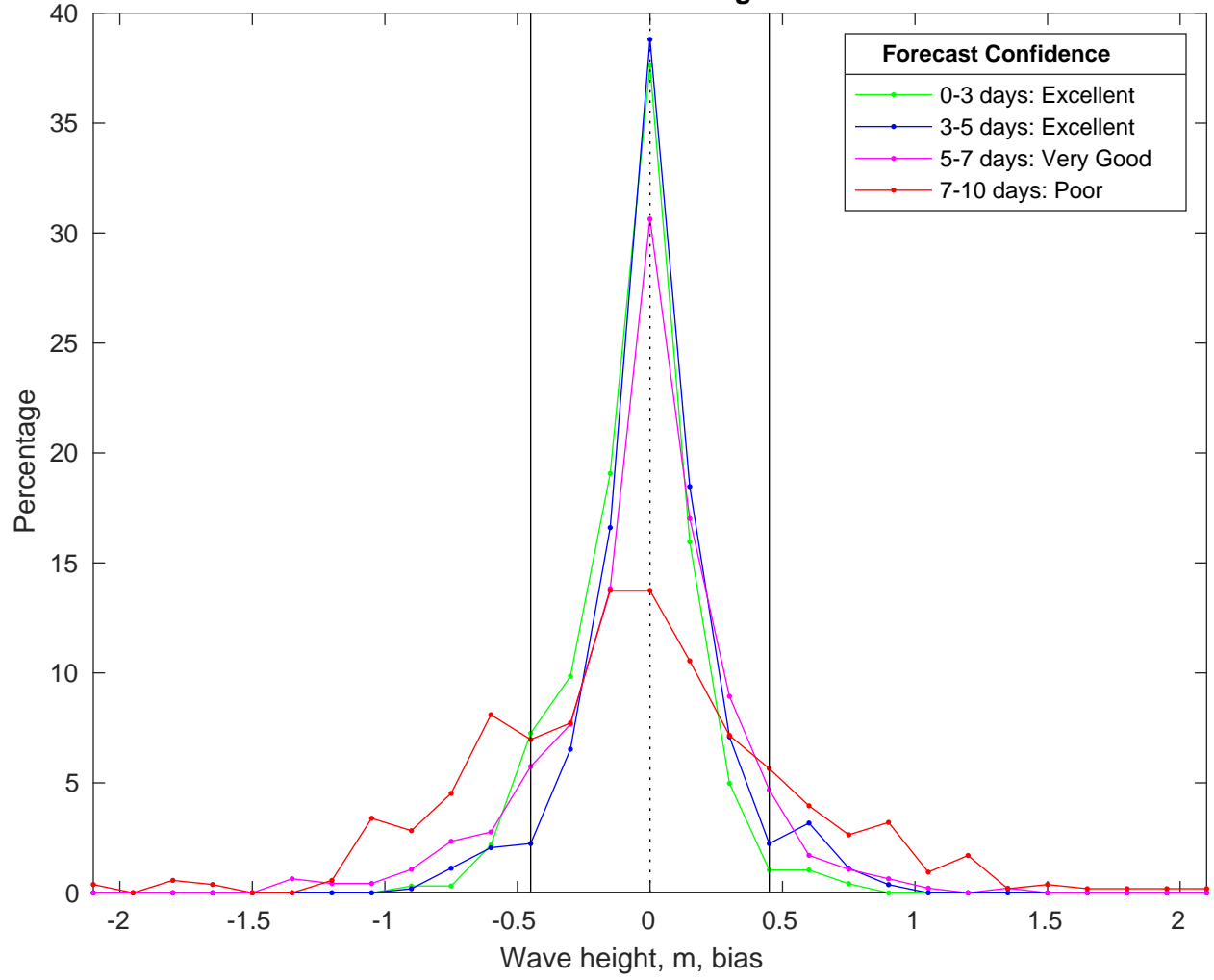
NDBC 41013 vs CMEMS Waves Bias Histogram: 10-Feb-2025
