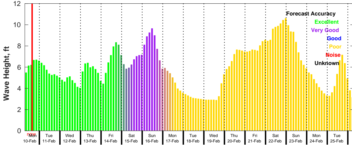
GFS Wave Forecast for NDBC 41013 from 10-Feb-2025 07:00:00 to 26-Feb-2025 07:00:00
