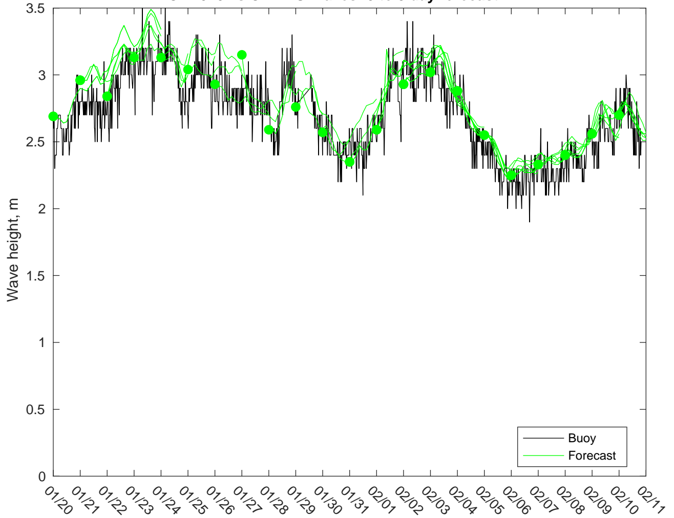
NDBC 41040 vs CMEMS Waves: 0 to 3 day forecast
