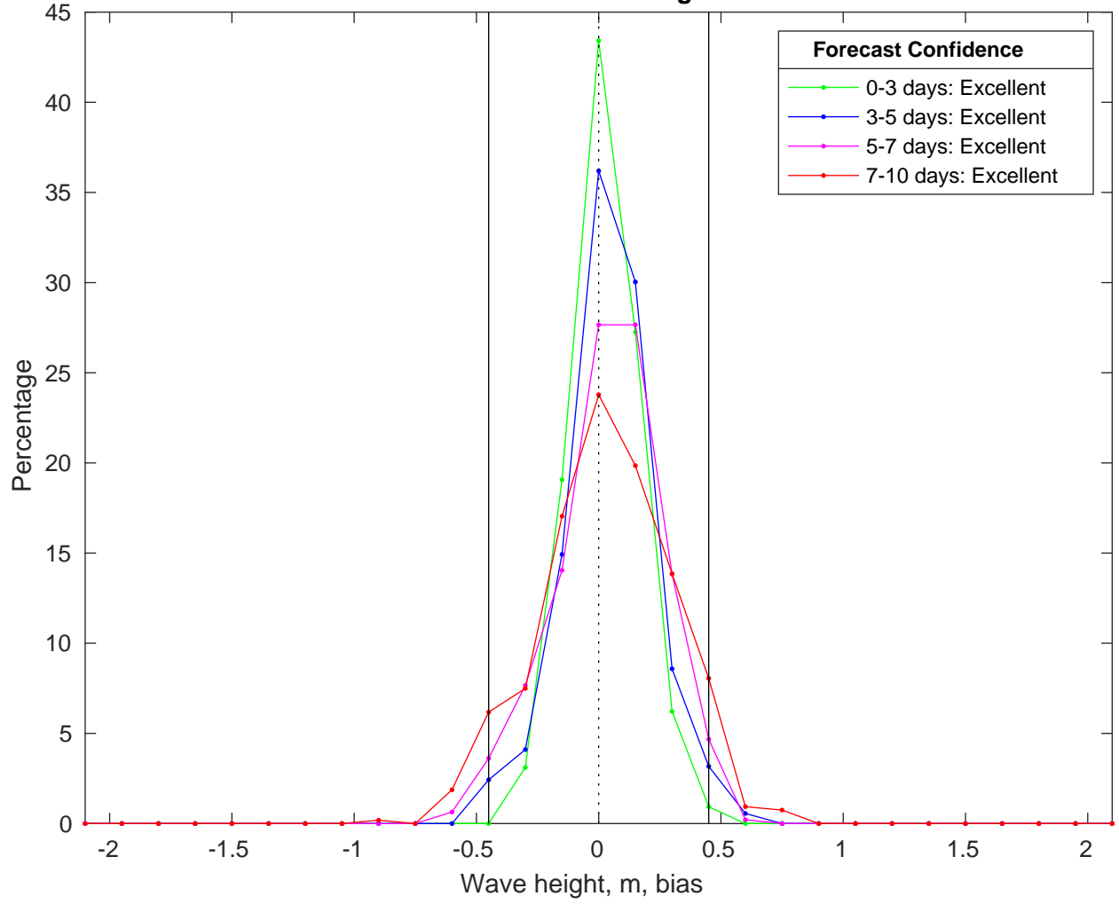
NDBC 41040 vs CMEMS Waves Bias Histogram: 10-Feb-2025
