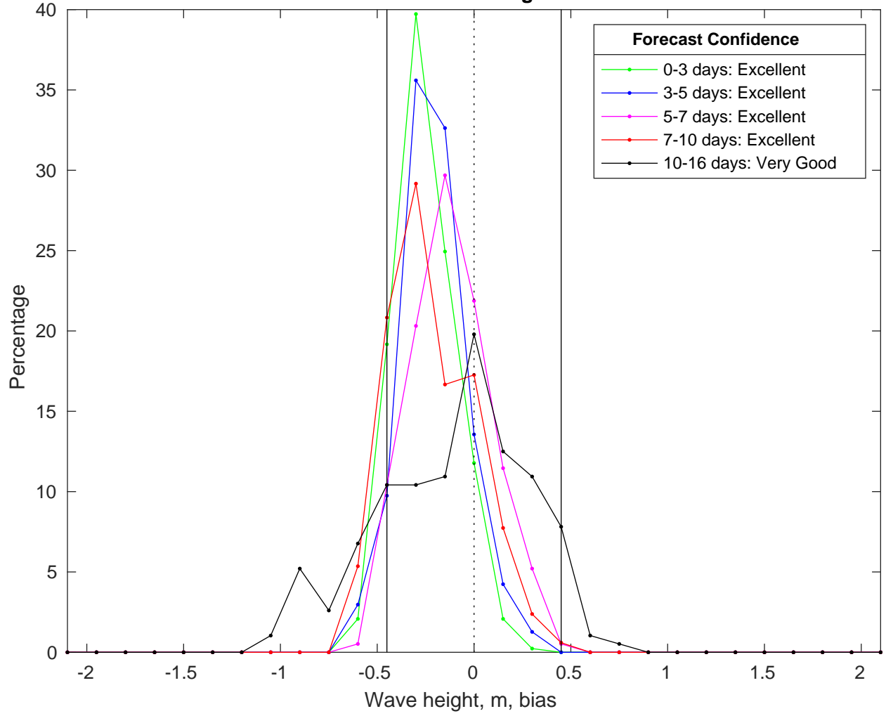
NDBC 41040 vs GFS Waves Bias Histogram: 10-Feb-2025
