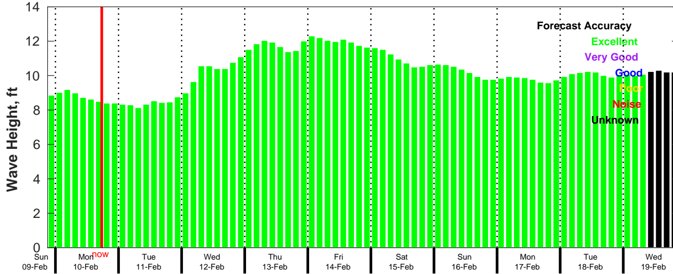
CMEMS Wave Forecast for NDBC 41040 from 09-Feb-2025 21:00:00 to 19-Feb-2025 21:00:00
