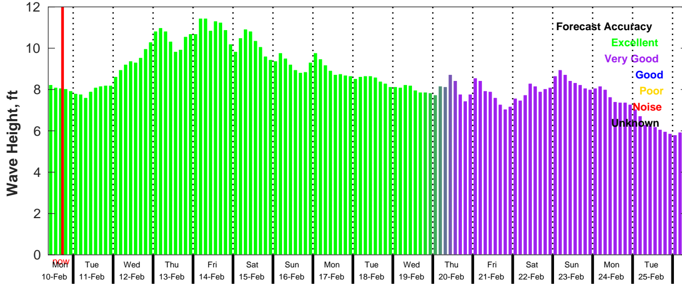
GFS Wave Forecast for NDBC 41040 from 10-Feb-2025 09:00:00 to 26-Feb-2025 09:00:00
