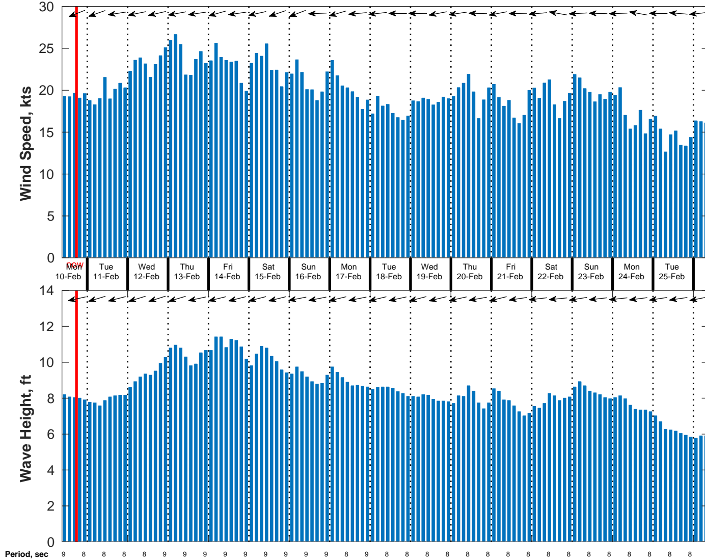
Wind & Wave Forecast for NDBC 41040 from 10-Feb-2025 09:00:00 to 26-Feb-2025 09:00:00
