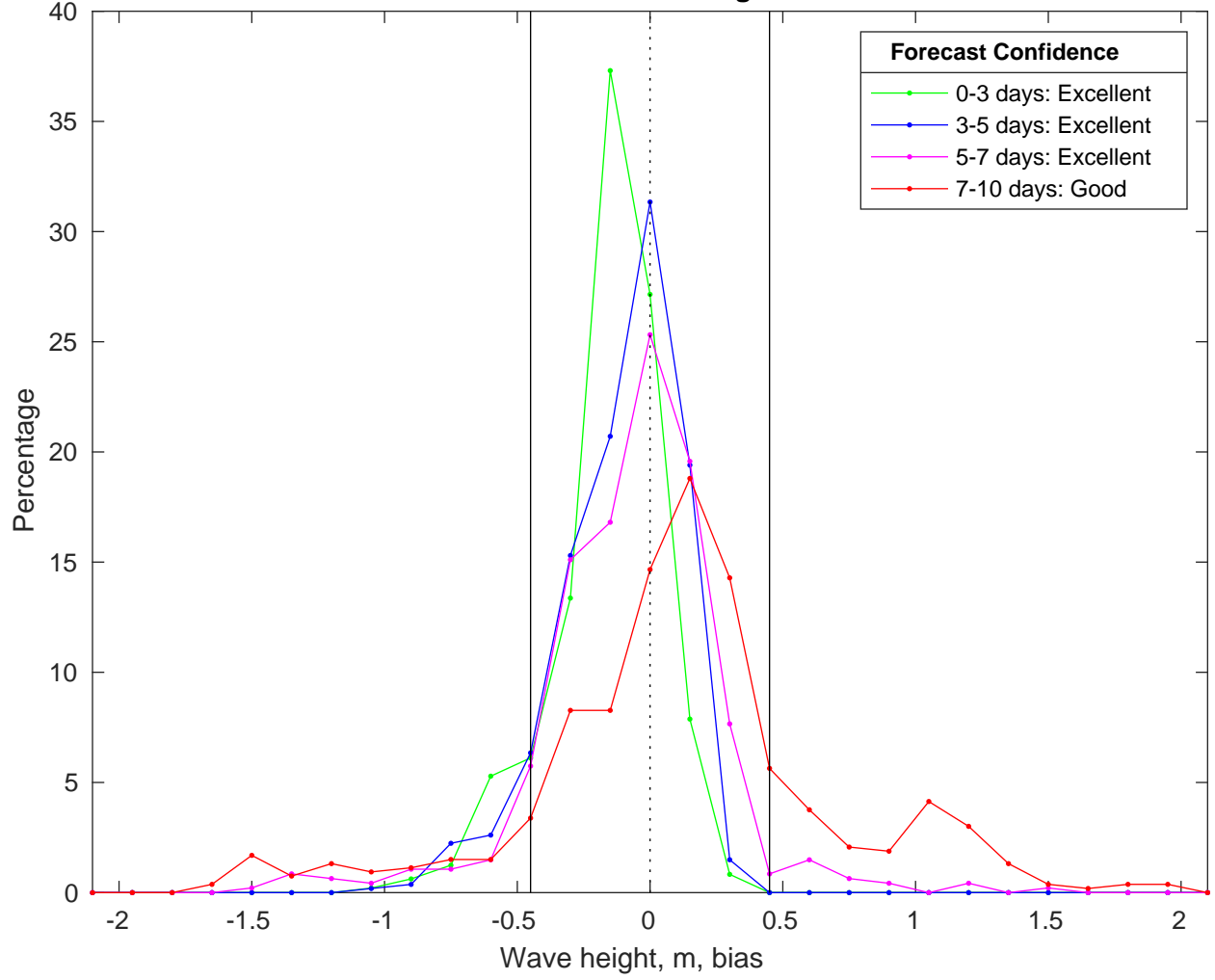
NDBC 42019 vs CMEMS Waves Bias Histogram: 10-Feb-2025
