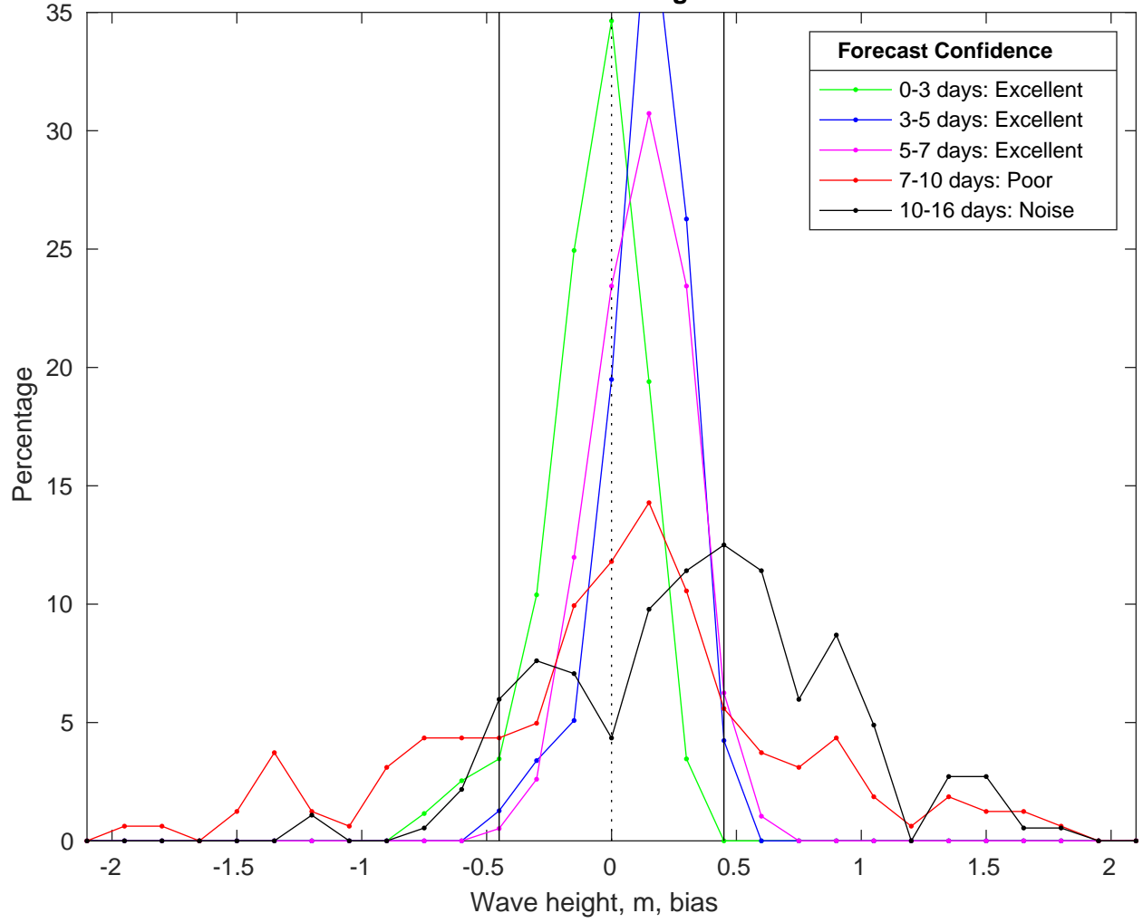
NDBC 42019 vs GFS Waves Bias Histogram: 10-Feb-2025
