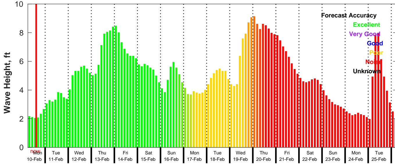
GFS Wave Forecast for NDBC 42019 from 10-Feb-2025 06:00:00 to 26-Feb-2025 06:00:00
