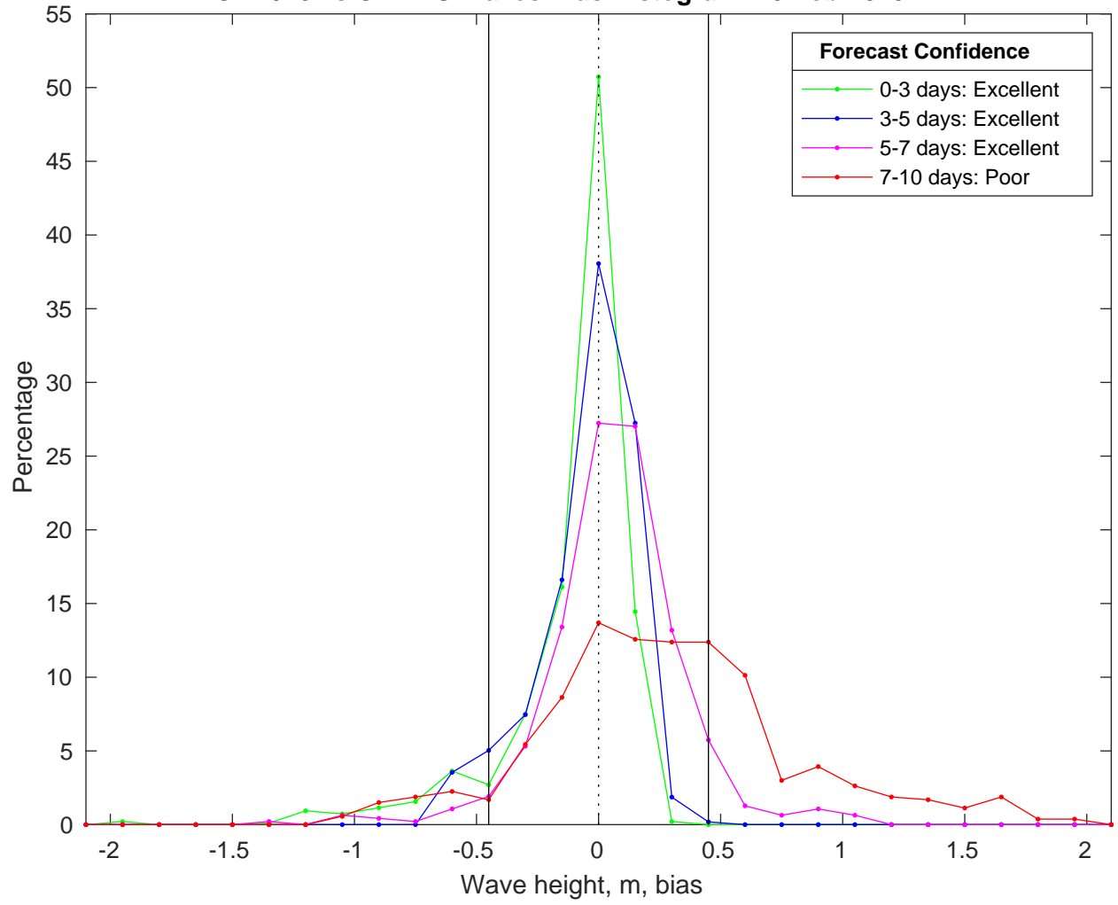
NDBC 42020 vs CMEMS Waves Bias Histogram: 10-Feb-2025
