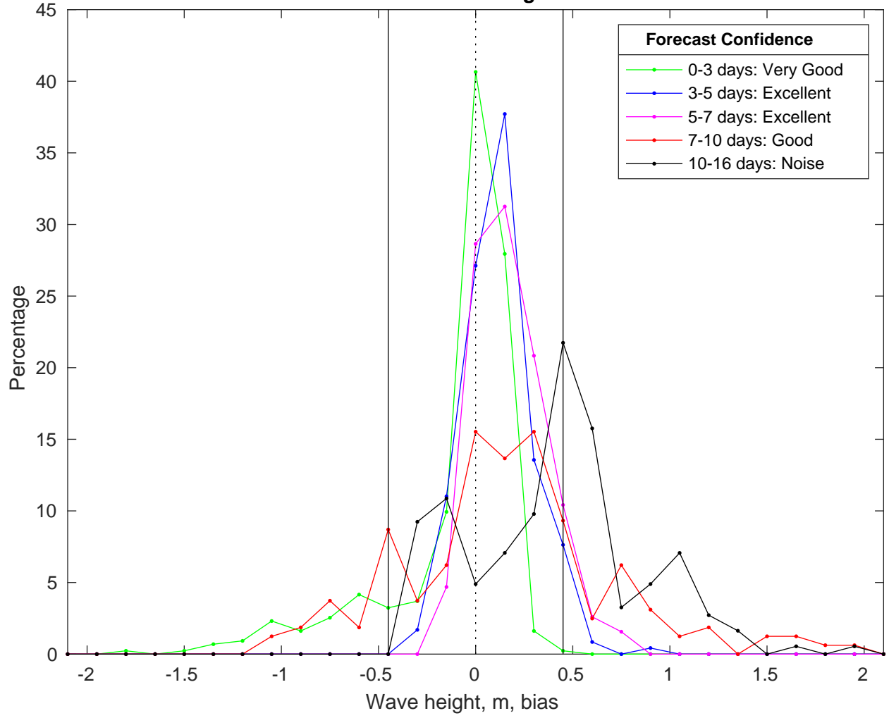
NDBC 42020 vs GFS Waves Bias Histogram: 10-Feb-2025
