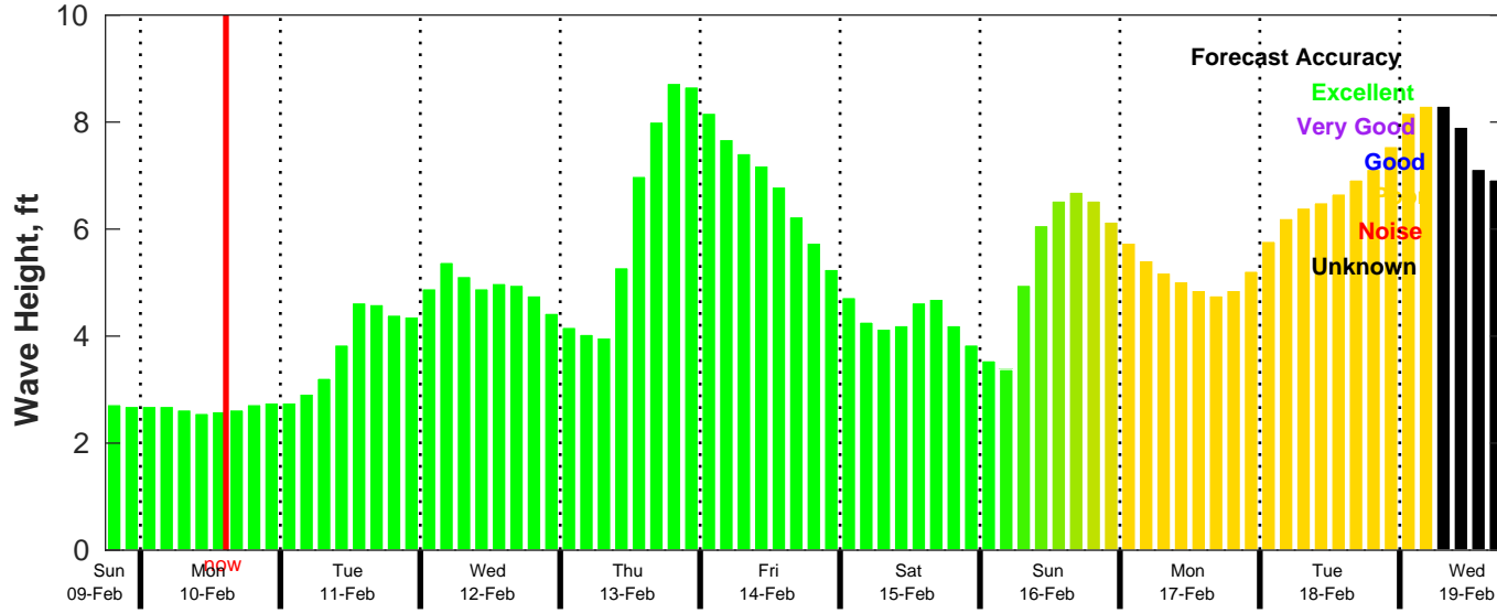
CMEMS Wave Forecast for NDBC 42020 from 09-Feb-2025 18:00:00 to 19-Feb-2025 18:00:00
