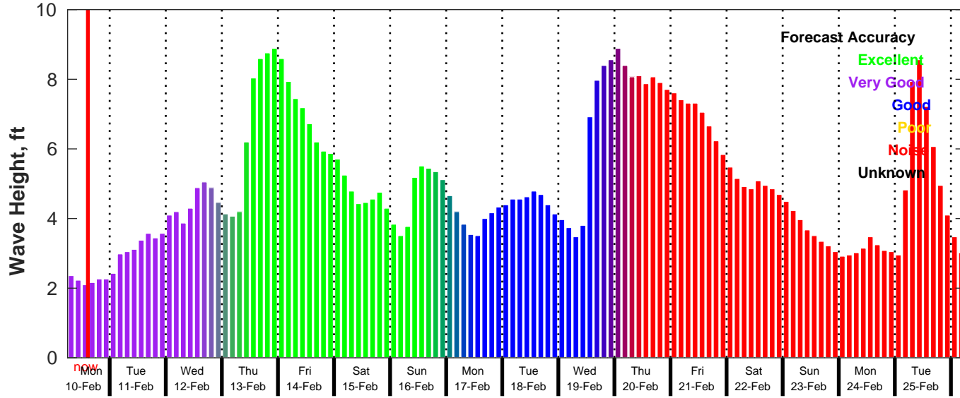
GFS Wave Forecast for NDBC 42020 from 10-Feb-2025 06:00:00 to 26-Feb-2025 06:00:00
