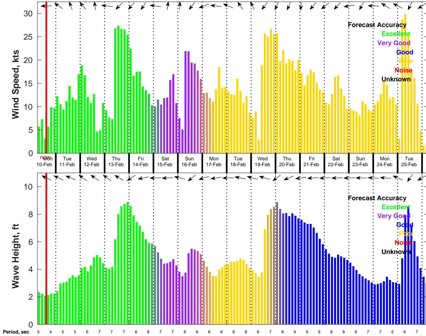
Wind & Wave Forecast for NDBC 42020 from 10-Feb-2025 06:00:00 to 26-Feb-2025 06:00:00
