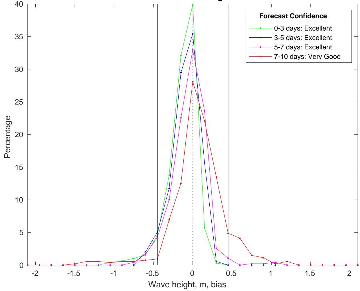
NDBC 42035 vs CMEMS Waves Bias Histogram: 10-Feb-2025
