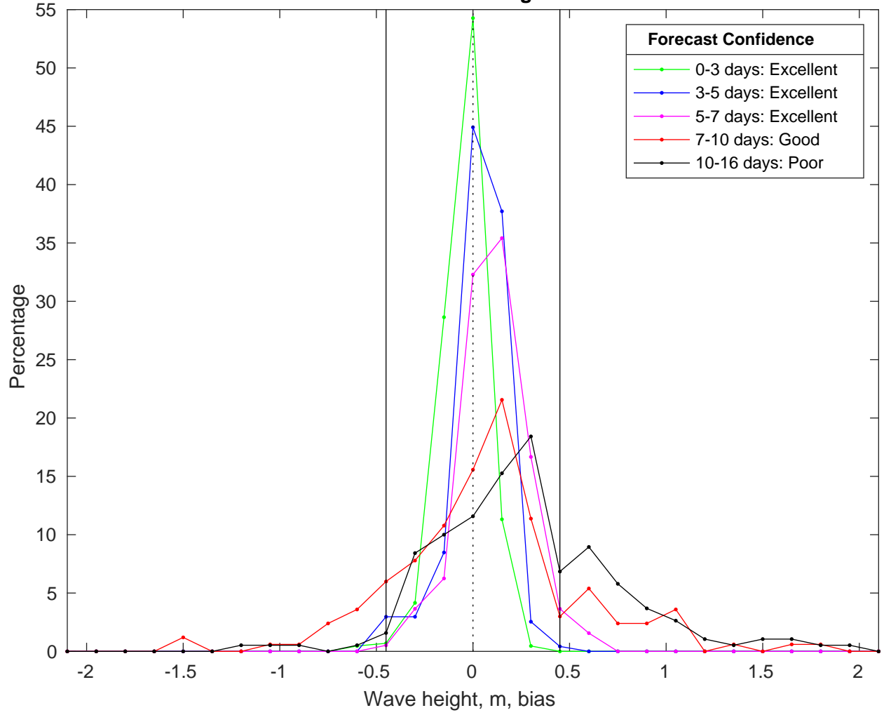
NDBC 42035 vs GFS Waves Bias Histogram: 10-Feb-2025
