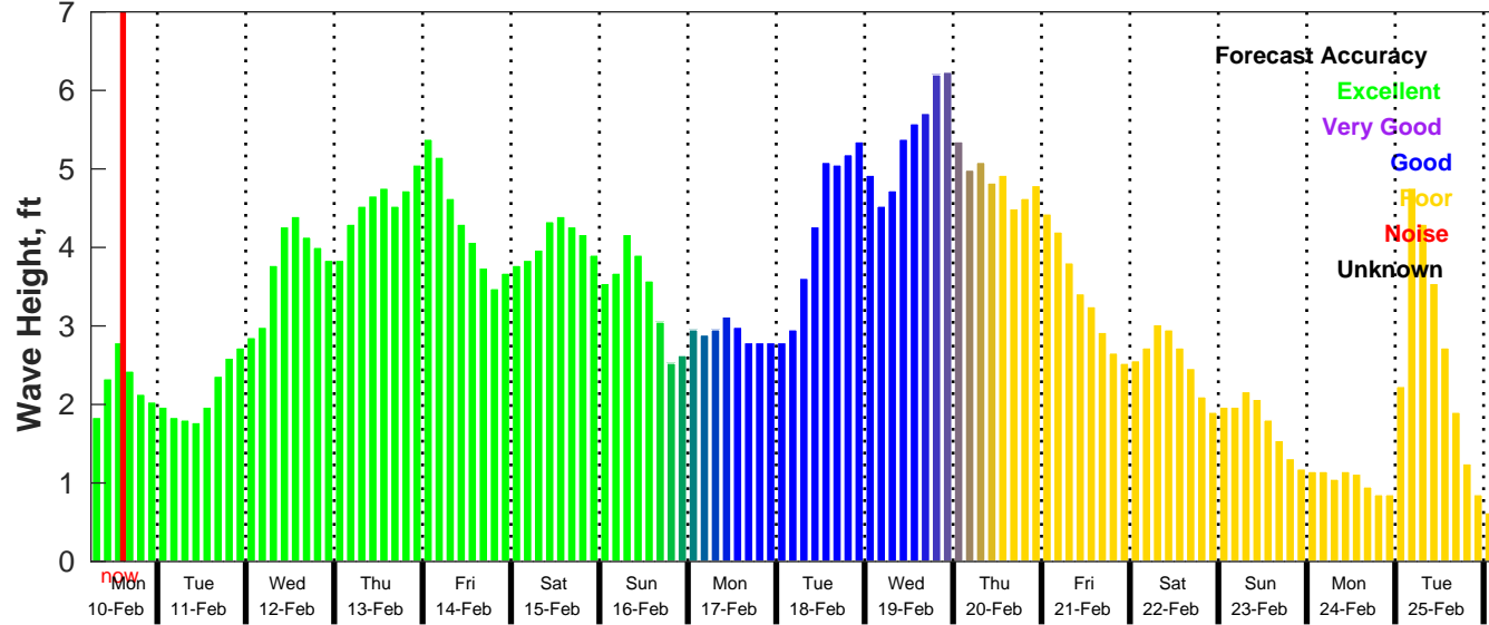
GFS Wave Forecast for NDBC 42035 from 10-Feb-2025 06:00:00 to 26-Feb-2025 06:00:00
