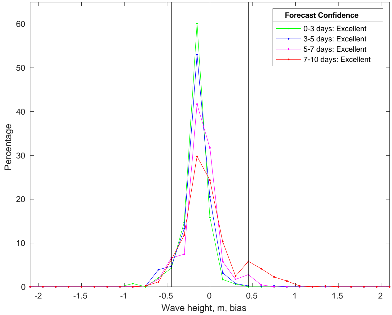
NDBC 42036 vs CMEMS Waves Bias Histogram: 10-Feb-2025
