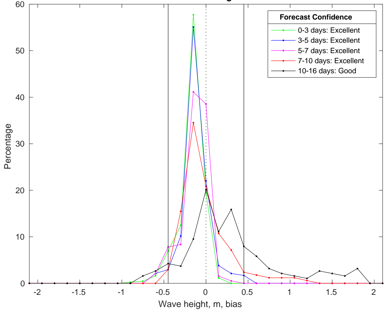
NDBC 42036 vs GFS Waves Bias Histogram: 10-Feb-2025
