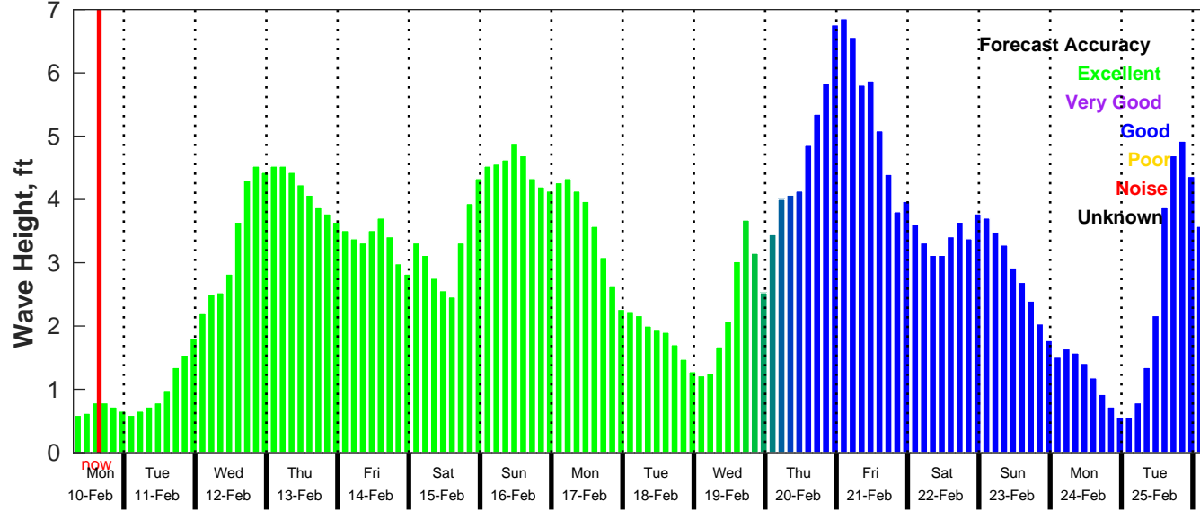
GFS Wave Forecast for NDBC 42036 from 10-Feb-2025 07:00:00 to 26-Feb-2025 07:00:00
